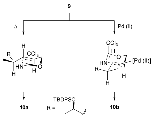
Fig. 1 Transition states for the thermal and palladium catalysed rearrangement of 9 .
