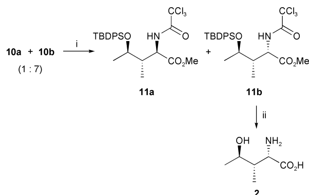
Scheme 3 Reagents and conditions: i. \text{O}_3 , NaOH, MeOH, -78^\circ\text{C} , 74%; ii. 6 M HCl, \Delta , 24 h, 88%.
